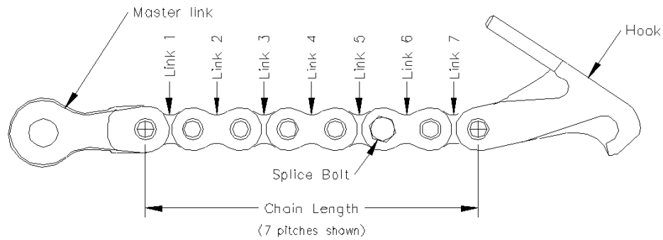
CHAIN ASSEMBLY
